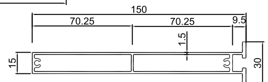
KU-429 1.587KG/M
