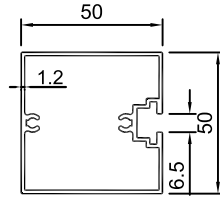
UR-167 0.845kg/m 232.9mm
