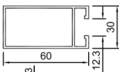
SKC-027 0.797kg/m 233.9mm
