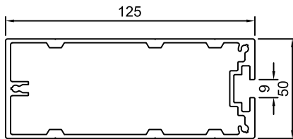
TKS-125 2.693kg/m 396.5mm
