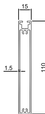
HM-023 ??: 1.169kg/m ????: 278.5mm
